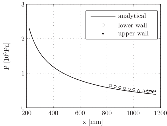
Figure 1: Typical static pressure axial evolution throughout the whole nozzle divergent ( p_0=4.2 bar)
