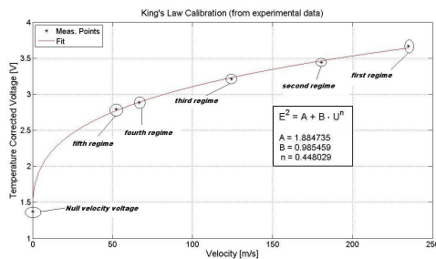
Figure 10: Unique Calibration Law Example
