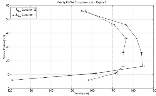
Figure 16: Velocity Profiles - H.W. Measures
