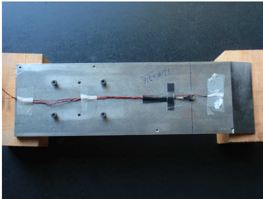
Figure 6: The accelerometer used for mechanical-vibrations measurements glued on the flat plate
