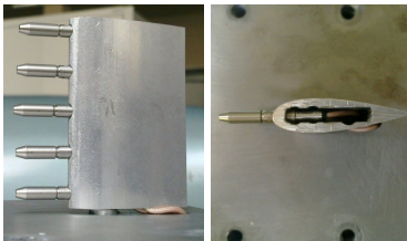
Figure 7: Manufactured 5 Probes Support
