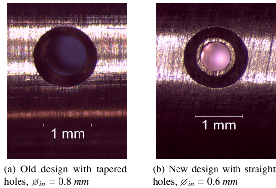
Figure 7: Inlet holes of the static pressure probe
