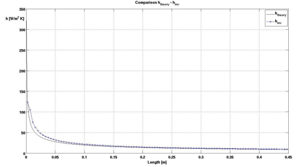
Figure 1: Theory - IHCP solution Comparison
