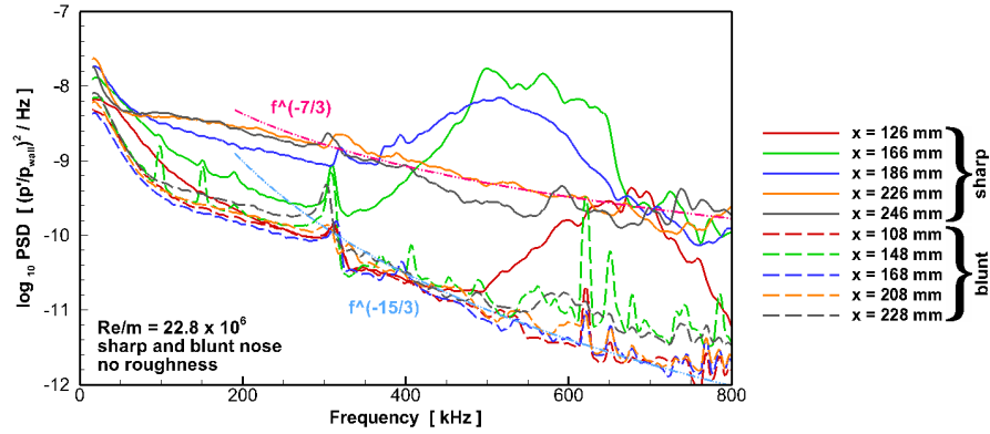
Figure 3: Nose bluntness effect on second modes
