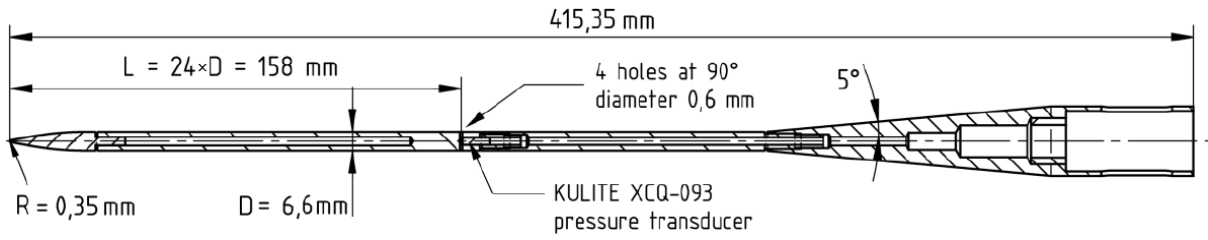
Figure 3: Static pressure probe following the design of Nagamatsu ([9])
