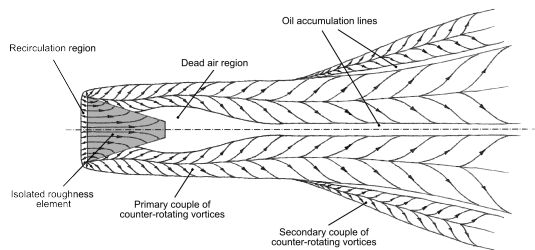
Figure 10: Vortex topology
