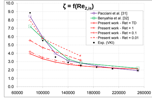
Figure 9: T106C mass-averaged kinetic losses (abscissa: Re_{2,is} , ordinate: \zeta )
