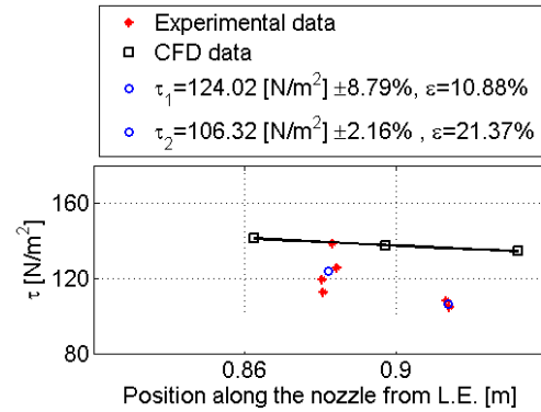
Figure 4: Measured shear/stress values at two different locations ( M_\infty = 1.9 )
