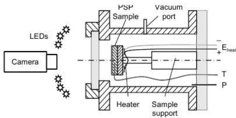
Figure 10: Sketch of the calibration setup
