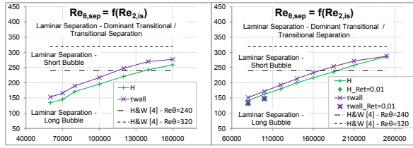
Figure 16: Re_{\theta,sep} through the Re_{2,is} range for T108 (left) and T106C (right) (abscissa: Re_{2,is} , ordinate: Re_{\theta,sep} )
