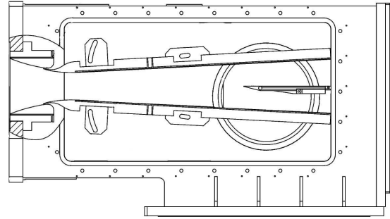
Figure 7: The flat plate with the accelerometer in the test section
