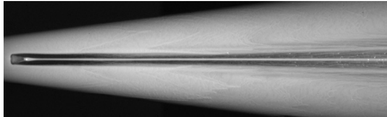
(b) Oil visualization on a blunt 2.5mm cone, ramp k=0.9\text{mm} , Re=18E6/m
