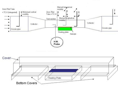
Figure 3: Test Section and Measuring Tools Installation Sketch (Courtesy of ULB)
