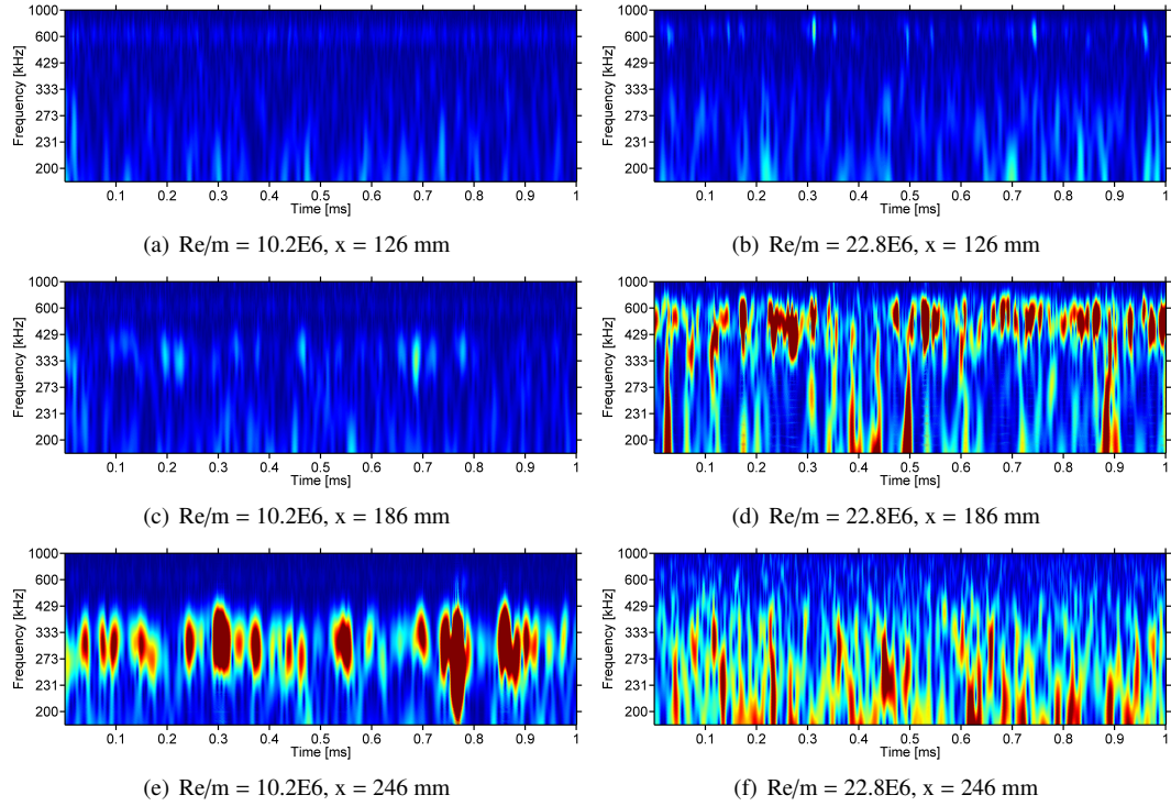
Figure 5: Wavelet analysis for different Reynolds number and sensors location
