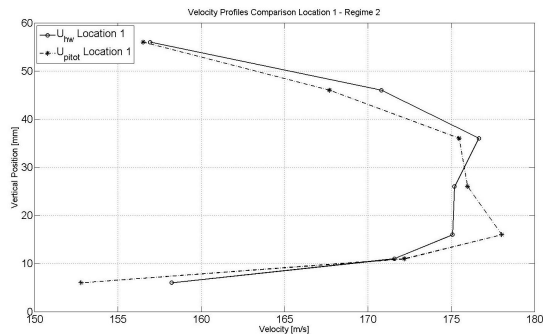
Figure 18: Velocity Profiles - Location 1, H.W. - Pitot Comparison
