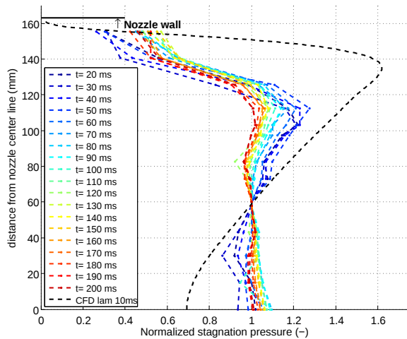
Figure 13: Unsteady normalized stagnation pressure profile at x = -1500 mm
