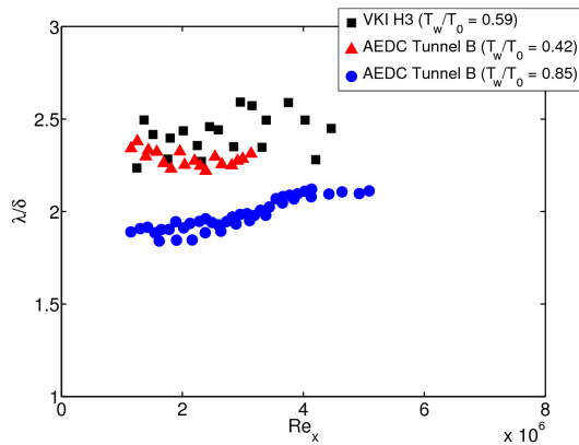
Figure 4: Approximate wavelength of second modes (replotted from Stetson and Kimmel [12])
