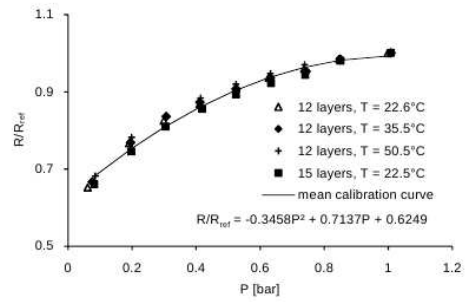
Figure 11: Calibration of binary PSP for different sample temperature and paint thickness (lifetime method)
