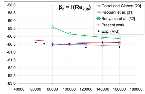
Figure 6: T108 mass-averaged outlet flow angle (abscissa: Re_{2,is} , ordinate: \beta_2 )
