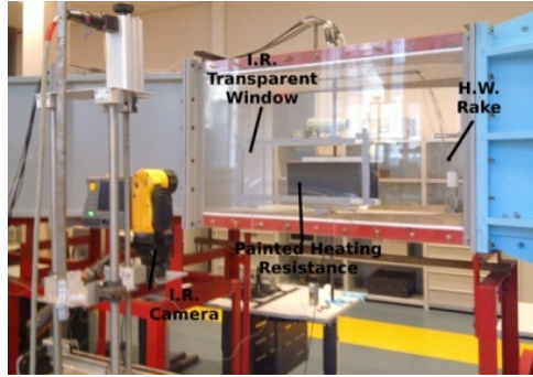
Figure 4: I.R. Low Speed Experiments setup
