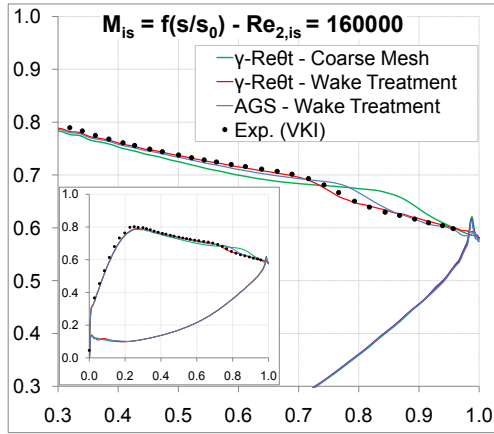
Figure 4: T108 comparison of \gamma\text{-}\widetilde{Re}_{\theta t} model and AGS criterion at Re_{2,is} = 160000 , M_{2,is} = 0.6 and Tu_1 = 0.9\% (abscissa: s/s_0 , ordinate: M_{is} )
