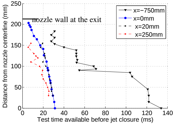
Figure 15: Jet closure time for various locations along the nozzle
