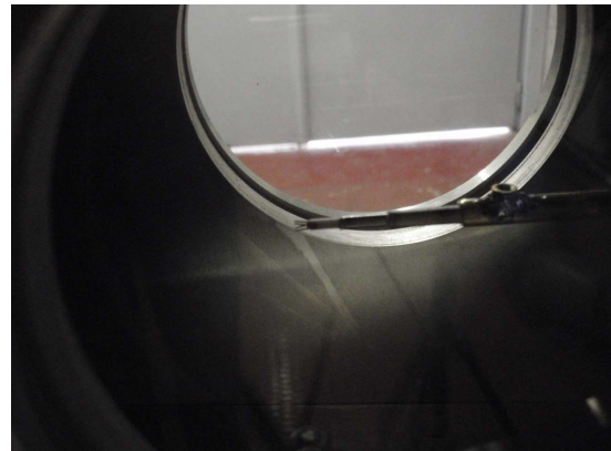
Figure 5: The double hot-wire in the test section
