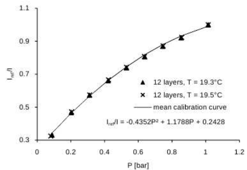
Figure 12: Calibration of binary PSP for different sample temperature and paint thickness (intensity method)
