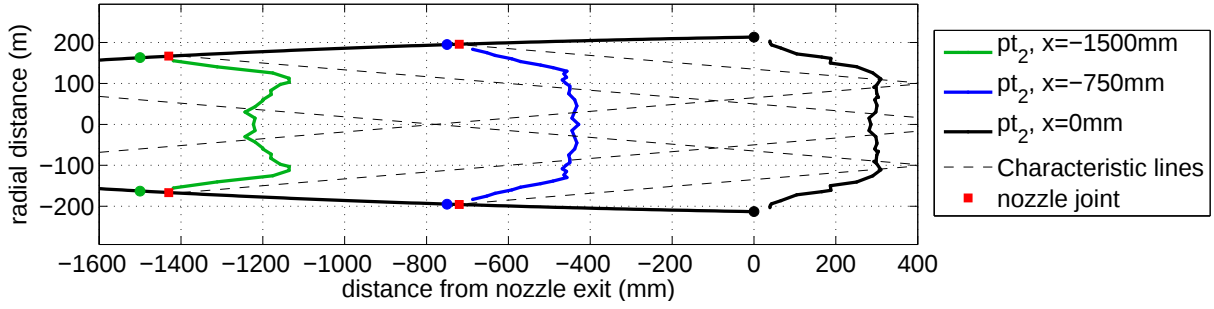
Figure 14: Boundary layer profiles through the nozzle with characteristic lines at Mach 12
