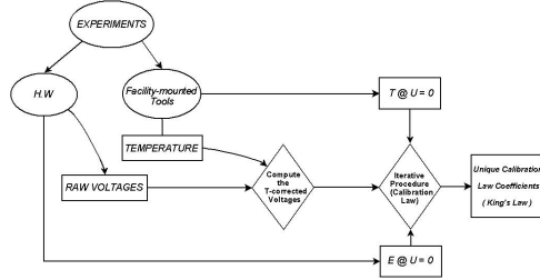
Figure 9: Unique Calibration Law Procedure Logical Scheme
