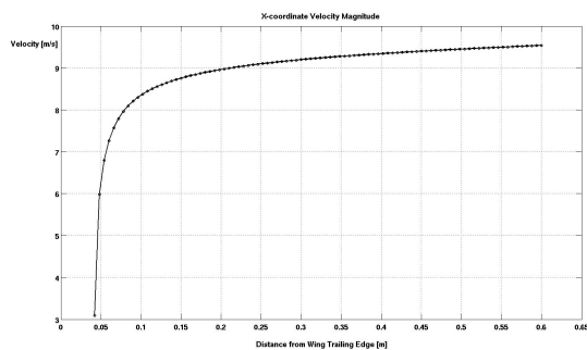
Figure 20: X-coordinate Velocity Plot
