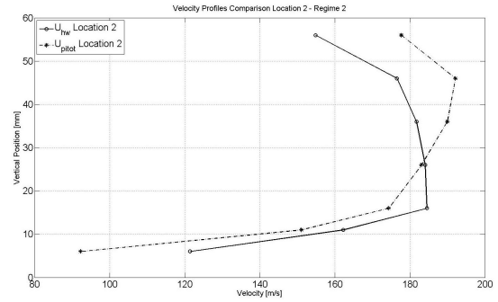
Figure 19: Velocity Profiles - Location 2, H.W. - Pitot Comparison
