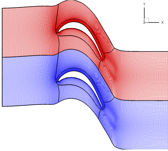
Figure 2: Mesh topology of T106C ( \Psi = 1.24 )
