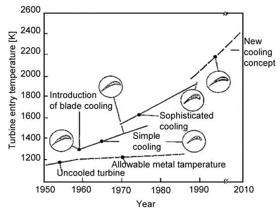
Figure 1: Variation of turbine entry temperature and the allowable metal temperature over several decades[1].
