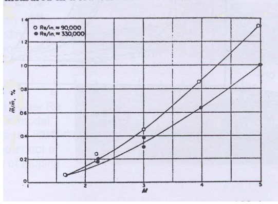
Figure 9: Variation of mass-flow fluctuations with free-stream Mach number, [5]
