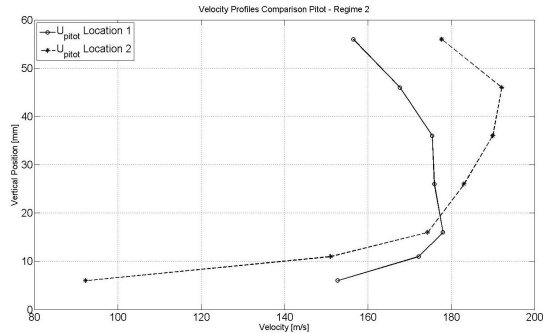
Figure 17: Velocity Profiles - Pitot Measures
