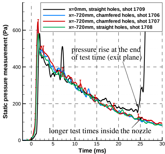
Figure 8: Measured static pressure
