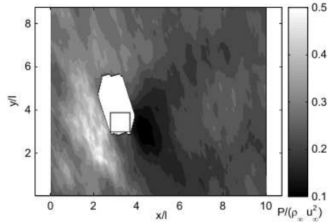
Figure 15: PSP map of the static pressure field around a single roughness element in a M_\infty = 1.8 flow, l = 4 \text{ mm} (lifetime method)
