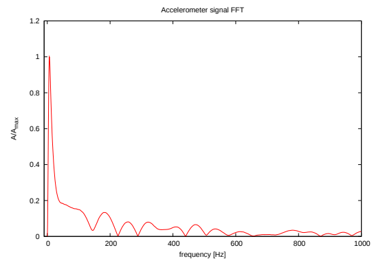
Figure 8: Frequency spectrum of mechanical vibrations of a flat plate in CT2
