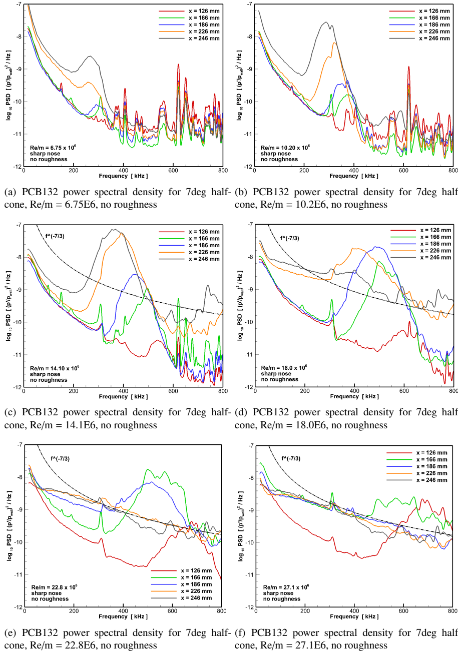
Figure 2: Second mode instabilities on a 7deg half-cone
