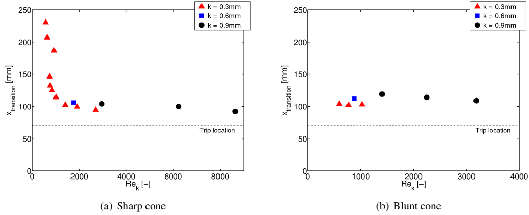
Figure 8: Roughness transition location vs Reynolds number
