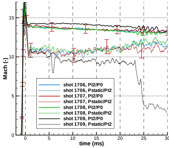
Figure 9: Free-stream Mach number determined from P_{t2}/P_0 and P_{static}/P_{t2}
