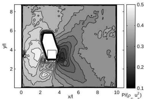
Figure 14: PSP map of the static pressure field around a single roughness element in a M_\infty = 1.8 flow, l = 4 \text{ mm} (intensity method)
