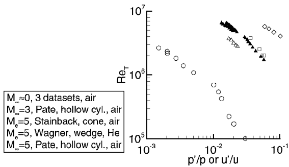
Figure 1: Transition Reynolds number data plotted as a function of the measured disturbance levels ([4])
