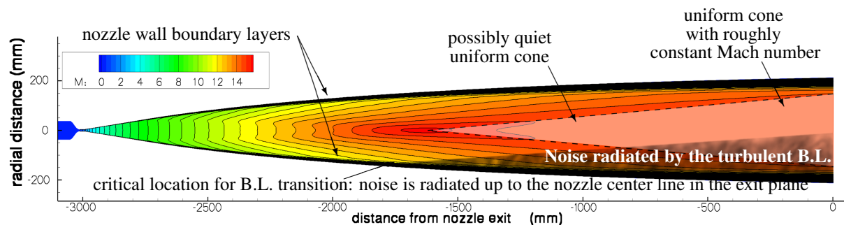
Figure 10: CFD prediction of Mach number in the nozzle and sound radiation by the boundary layers
