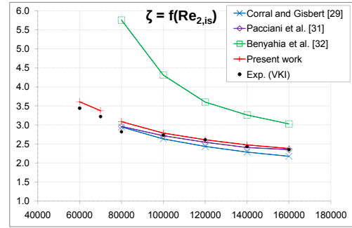
Figure 5: T108 mass-averaged kinetic losses (abscissa: Re_{2,is} , ordinate: \zeta )
