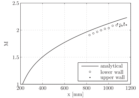
Figure 2: Typical Mach number axial evolution throughout the whole nozzle divergent ( p_0=4.2 bar)
