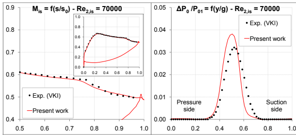
Figure 8: T108 isotropic Mach number distribution and wake profile at Re_{2,is} = 70000 (left abscissa: s/s_0 , left ordinate: M_{is} , right abscissa: y/g , right ordinate: \Delta P_{01}/P_{01} )
