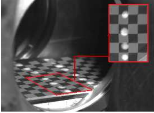
Figure 3: Oil dots on a checkered area for the reference image
