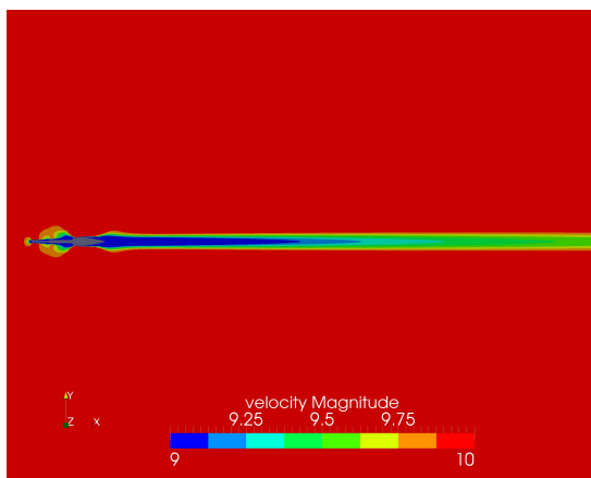
Figure 21: CFD-computed Velocity Contour Plot
