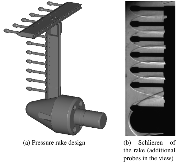
Figure 5: Pressure rake for boundary layer characterization
