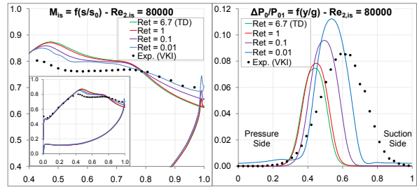
Figure 12: T106C isentropic Mach number distribution and wake profile with Re_t effect at Re_{2, is} = 80000 (left abscissa: s/s_0 , left ordinate: M_{is} , right abscissa: y/g , right ordinate: \Delta P_{01}/P_{01} )
