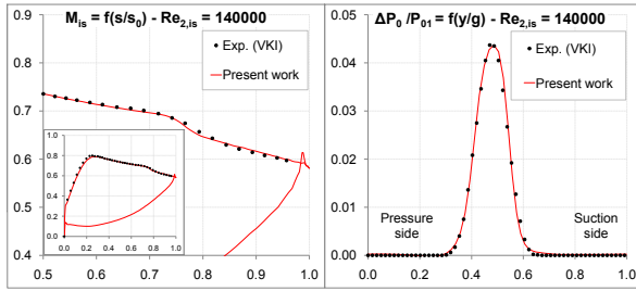
Figure 7: T108 isotropic Mach number distribution and wake profile at Re_{2,is} = 140000 (left abscissa: s/s_0 , left ordinate: M_{is} , right abscissa: y/g , right ordinate: \Delta P_0/P_{01} )
