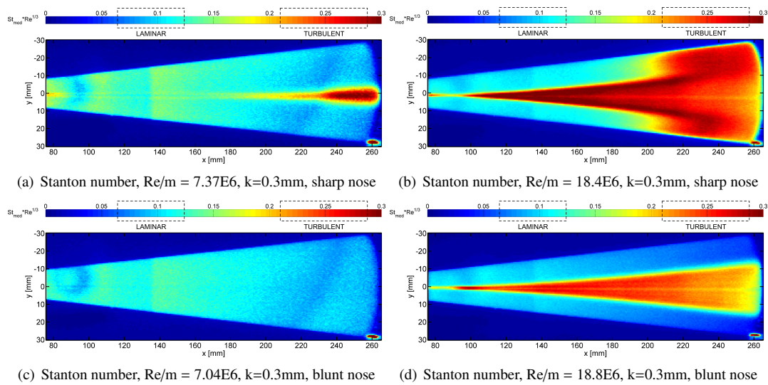
Figure 7: Infrared images on a 7deg half-cone
