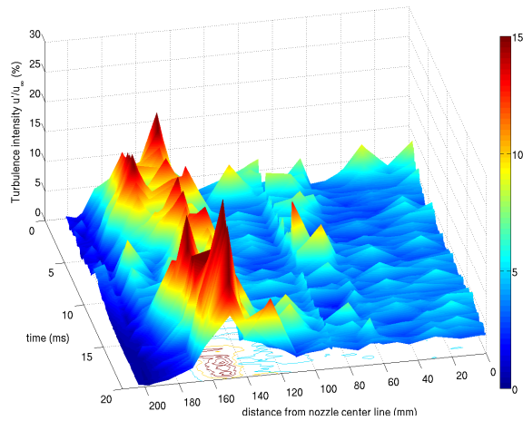
Figure 16: Turbulence intensities at the nozzle exit
