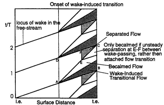
Figure 1: Time-space diagram of the turbulent spots (Schulte and Hodson [9])
