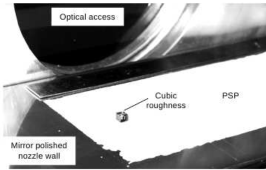
Figure 13: The PSP applied around a cubic roughness
