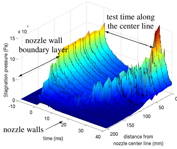
Figure 11: Stagnation pressure profile as a function of time at the nozzle exit for experiments at "Low" Reynolds (using N_2 )
