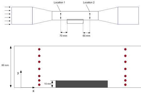
Figure 5: H-W. Traverses Experiments
