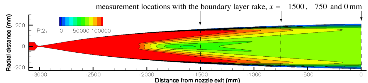
Figure 6: Measurement locations along the nozzle on top of CFD prediction of stagnation pressure p_{t2} for t=0 ms
