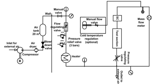
Figure 2: Facility Working Principle Diagram (Courtesy of ULB)
