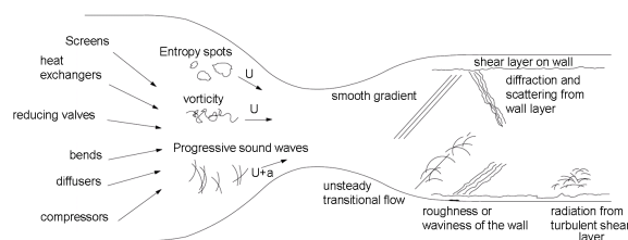
Figure 2: Free-stream disturbances in supersonic wind tunnels ([3])
