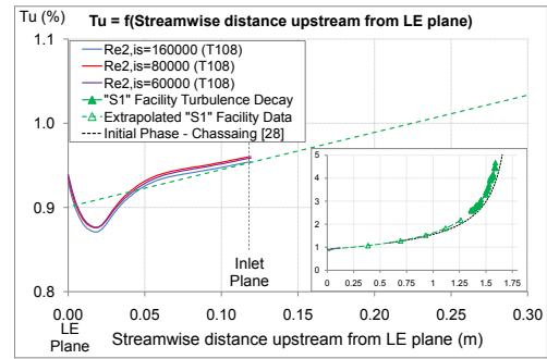
Figure 3: “S1” Decay of turbulence ahead of the cascade
