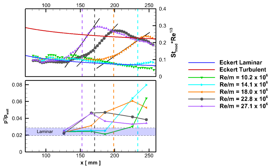
Figure 6: Natural transition and Pate correlation
