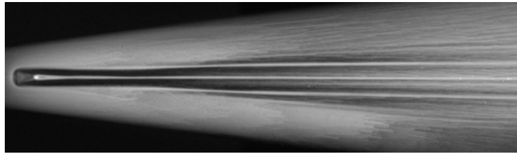
(a) Oil visualization on a sharp cone, ramp k=0.9\text{mm} , Re=18E6/m
