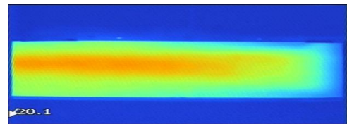
Figure 13: Cold Surface I.R. Image
