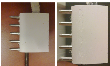
Figure 8: Manufactured 5 Probes Support (Plaster)
