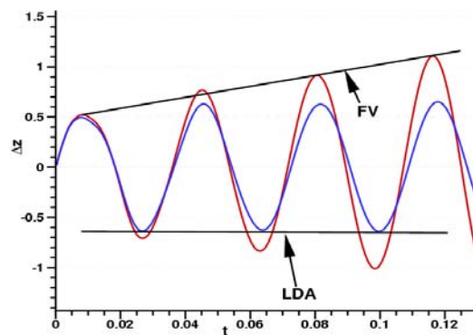
Figure 2 : AGARD 445.6 wing. Neutral regime. Deflection vs. time.
