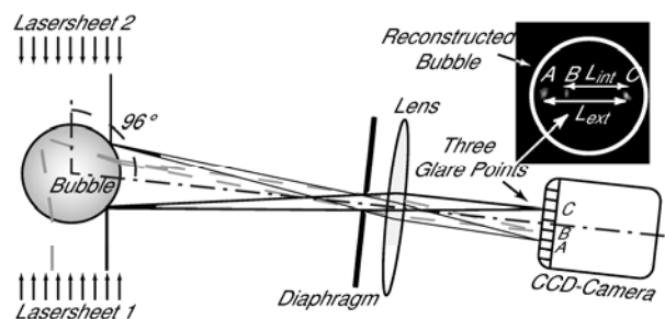
Figure 2: Extended GPVS setup
