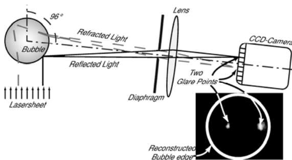
Figure 1: Basic GPVS setup
